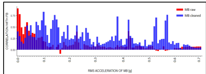
Figure 3. Correlation between FB and MB raw & MB cleaned RR signals. Bars represent means of correlation computed over binned values of RMSA. Cleaned MB data (blue) is more highly correlated with FB than raw MB data (red) for most values of RMSA.
